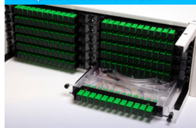
Variety of chassis fits up to 288 fibers in 1/3 the space of traditional LGX
